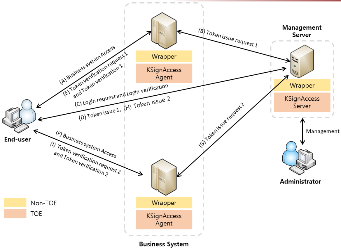
[Figure 1-1] end-user identification and authentication procedure
